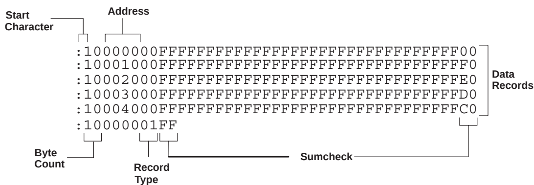
Figure A–1. Intel-Hex Object Format
