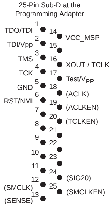
Figure 3–1. 25-Pin Sub-D at Programming Adapter
